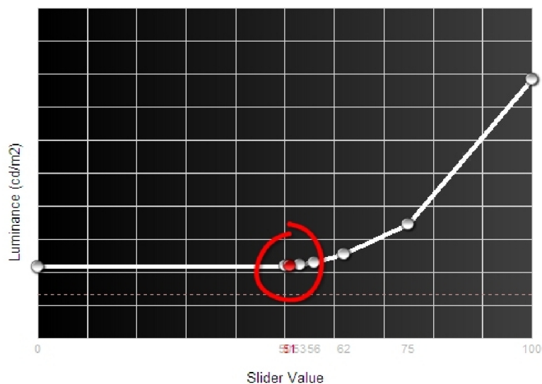
Brightness Setting Graph
