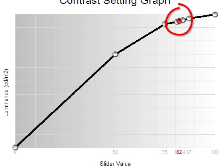
Contrast Setting Graph
